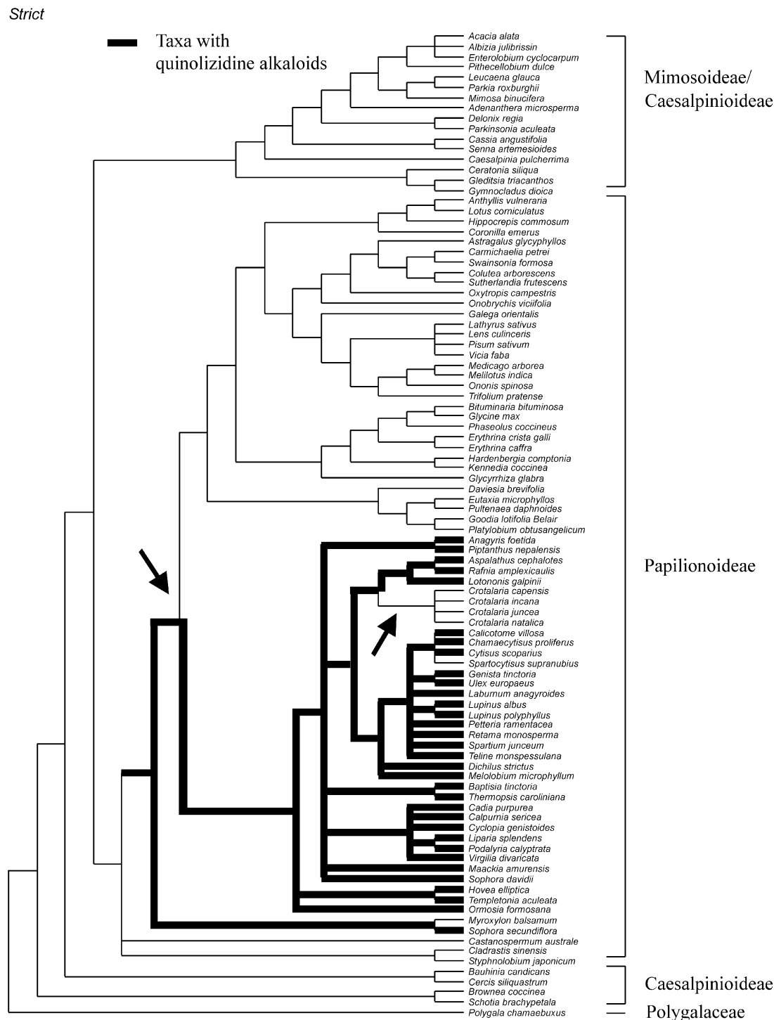
Fig. 1. Distribution of quinolizidine alkaloids in Fabaceae. MP-tree; strict consensus. Because the phytochemical analysis is still incomplete for some compounds or taxa, and since a few published findings may actually be wrong, inconsistencies should be interpreted with caution. The arrows point to critical bifurcations, splitting clades producing QA from those that do not produce QA. In case of Crotalaria , pyrrolizidine alkaloids replace QA as defence compounds.
